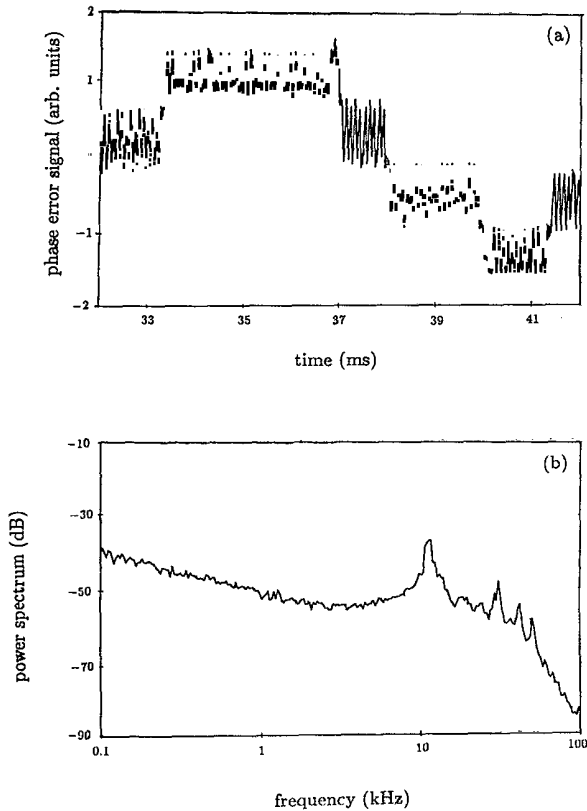
FIG. 8. Cycle slipping of a first-order PLL with time delay. (a) Temporal domain; (b) power spectrum.
