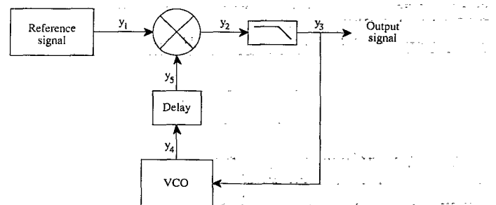
FIG. 3. First-order phase-locked loop with time delay.
