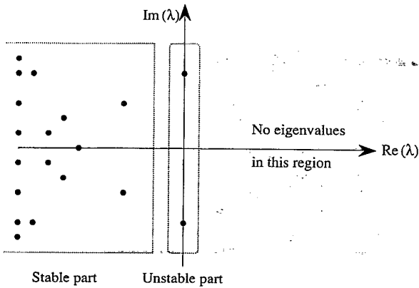
FIG. 2. Schematic representation of the spectrum of a delay-differential equation at an instability. The unstable part consists of those eigenvalues whose real part nearly vanishes whereas the infinity of eigenvalues of the stable part lie in a region separated by a finite distance from the unstable part.
