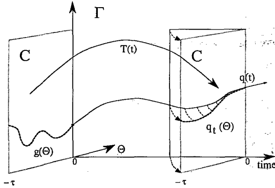
FIG. 1. Folding mechanism relating a history of q(t) \in \Gamma to a single element q_t \in \mathcal{C} .
