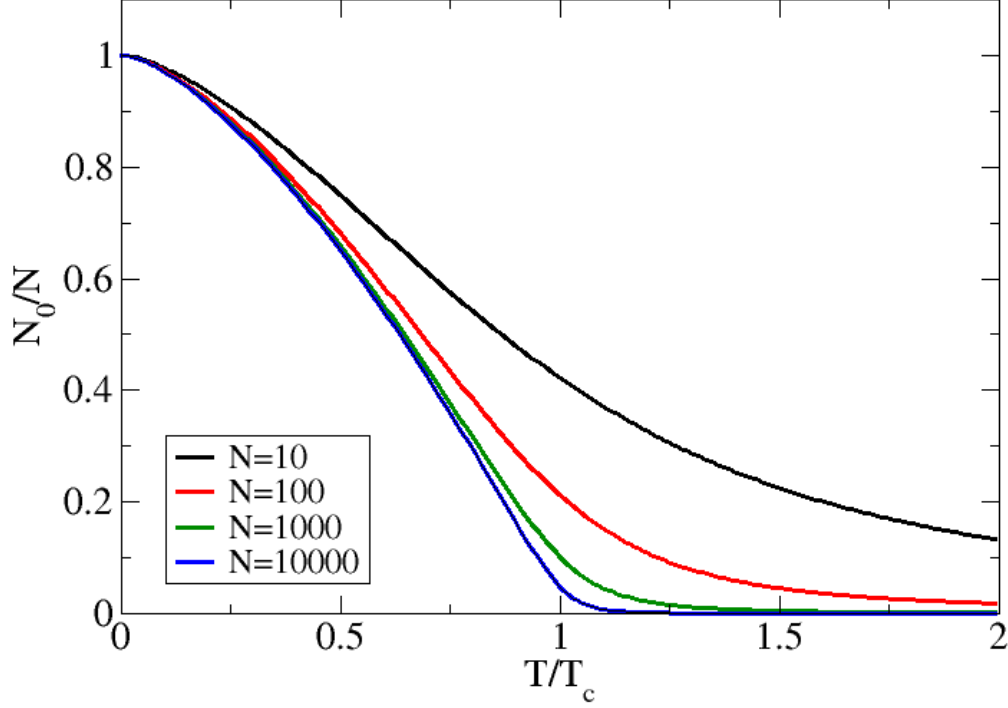
Figure 4.1: Condensed fraction of a homogeneous ideal Bose gas as a function of reduced temperature T/T_c^{(0)} with T_c^{(0)} given by Eq. (2.52) in the canonical ensemble for 10, 100, 1000 and 10000 particles calculated by Eq. (4.35).
