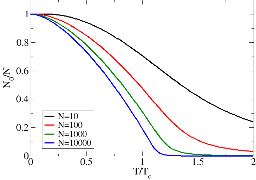
Figure 4.3: Condensed fraction of a 3D finite box as a function of reduced temperature T/T_c^{(0)} with T_c^{(0)} given by Eq. (2.52) in the canonical ensemble for 10, 100, 1000 and 10000 particles calculated by Eq. (4.35).
