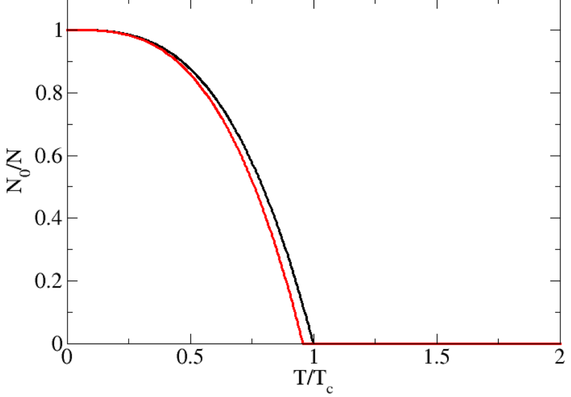
Figure 3.5: Condensate fraction of the isotropic three-dimensional harmonic trap as a function of reduced temperature T/T_c^{(0)} with T_c^{(0)} given by Eq. (2.62) in the thermodynamic limit. The black line corresponds to the non-interacting curve while the red line is the interacting plot - here we have that the interaction decreases the curve behavior, following the prevision given by the critical temperature calculation.
