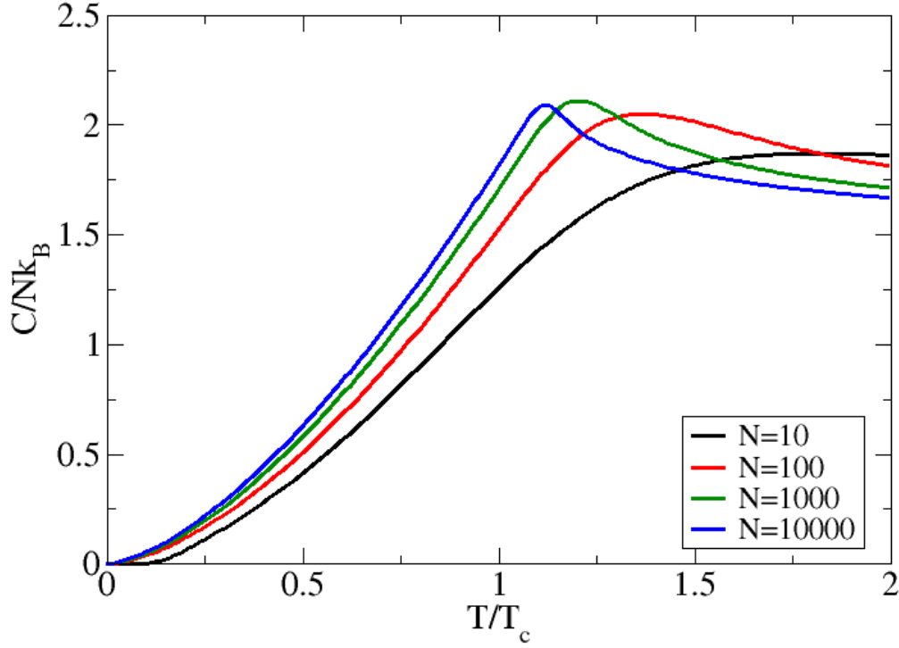
Figure 4.4: Heat capacity of a Bose gas in a 3D finite box as a function of reduced temperature T/T_c^{(0)} with T_c^{(0)} given by Eq. (2.52) in the canonical ensemble for 10, 100, 1000 and 10000 particles calculated by Eq. (4.42).
