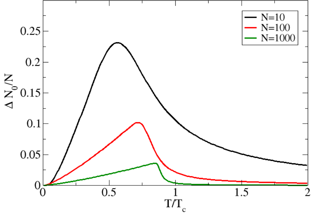
Figure 5.15: Ground state fluctuation for 10, 100, 1000 particles in a weakly interacting harmonic trap with gas parameter given by a_s n^{1/3} = 0.1 .
