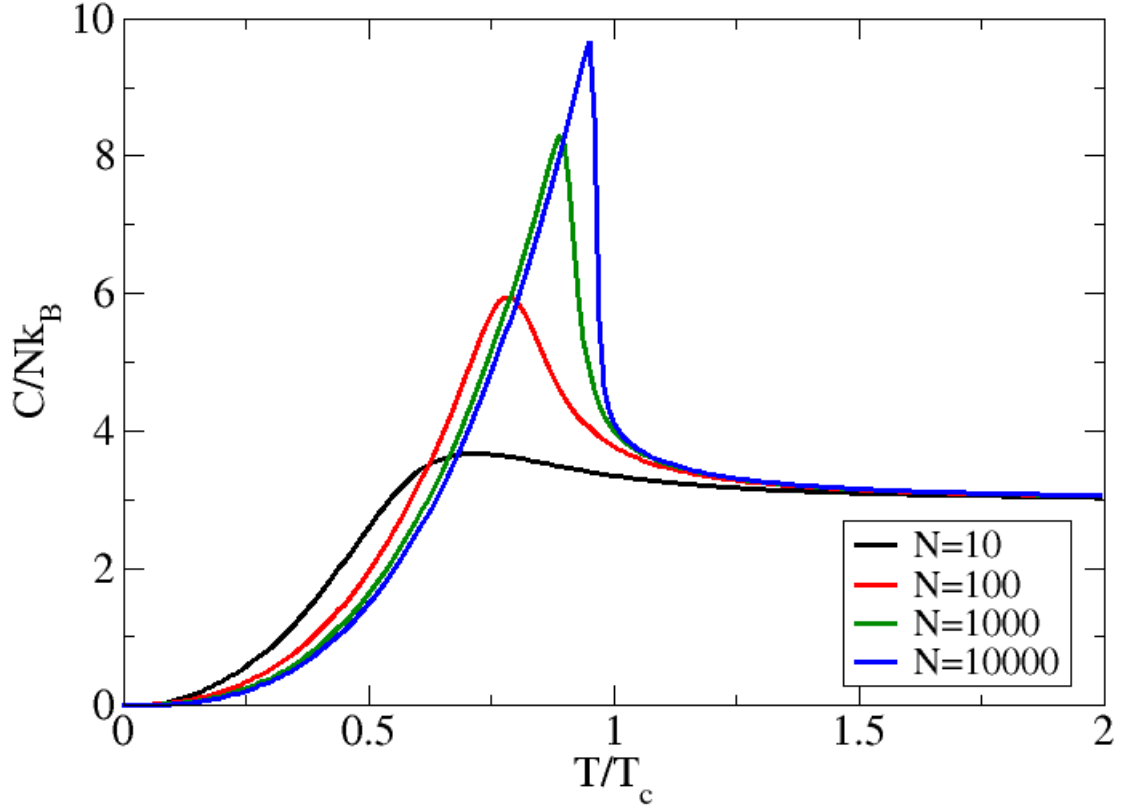
Figure 4.6: Heat capacity of a Bose gas in a 3D isotropic harmonic trap as a function of the temperature in the canonical ensemble for different numbers of particles N .
