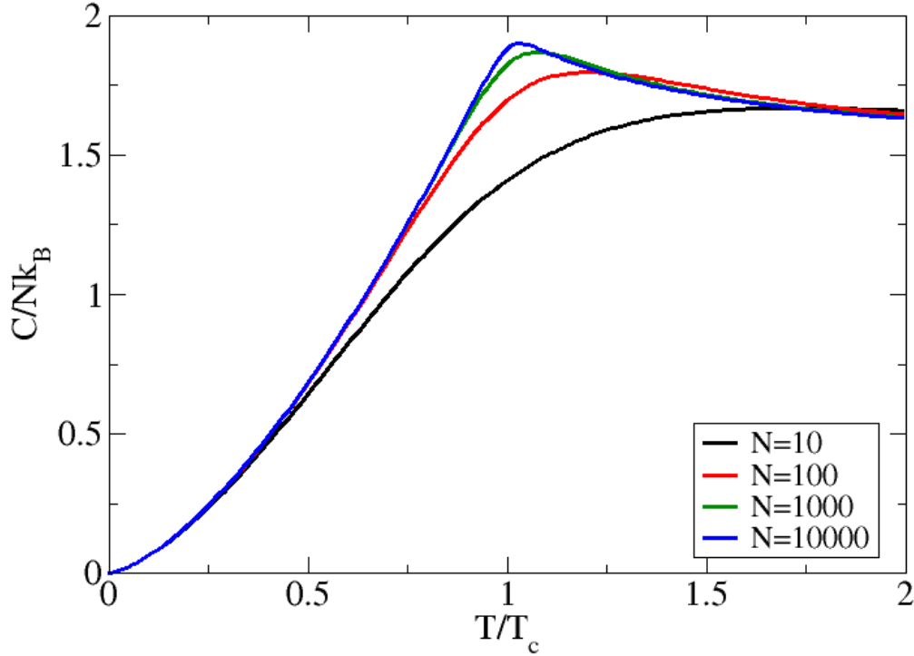
Figure 4.2: Heat capacity for a homogeneous 3D Bose gas as a function of reduced temperature T/T_c^{(0)} with T_c^{(0)} given by Eq. (2.52) in the canonical ensemble for 10, 100, 1000 and 10000 particles calculated by Eq. (4.42).
