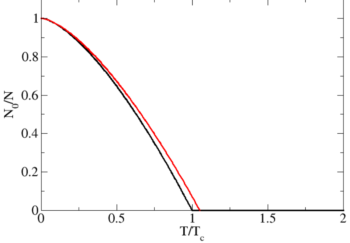
Figure 3.6: Condensate fraction of the isotropic three-dimensional finite box as a function of reduced temperature T/T_c^{(0)} with T_c^{(0)} given by Eq. (2.52) in the thermodynamic limit. The black line corresponds to the non-interacting curve while the red line is the interacting plot - here we have that the interaction decreases the curve behavior, following the prevision given by the critical temperature calculation.
