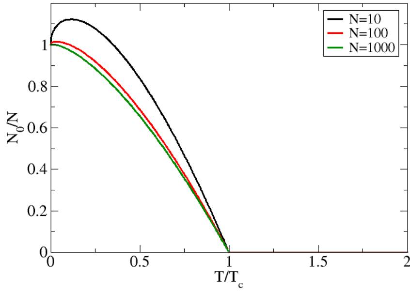
Figure 2.3: Condensate fraction for a three-dimensional finite box using the homogeneous semiclassical approximation calculated by Eq. (2.75) as a function of reduced temperature T/T_c^{(0)} with T_c^{(0)} given by Eq. (2.52) for different numbers of particles N . The brown line in zero corresponds to all plots after the critical point due to, independently of N , the condensate fraction being zero for high temperatures in the grand canonical ensemble. Here is clear that this semiclassical approximation for a box trap is not good enough to describe the finite-size correction, so we need to do a semiclassical treatment using the discrete energy representation.
