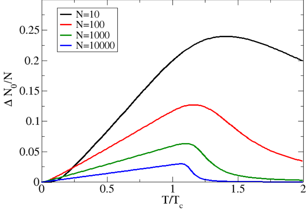
Figure 4.5: Ground-state fluctuation of a Bose gas in a 3D finite box as a function of reduced temperature T/T_c^{(0)} with T_c^{(0)} given by Eq. (2.52) in the canonical ensemble for 10, 100, 1000 and 10000 particles calculated by Eq. (4.39).
