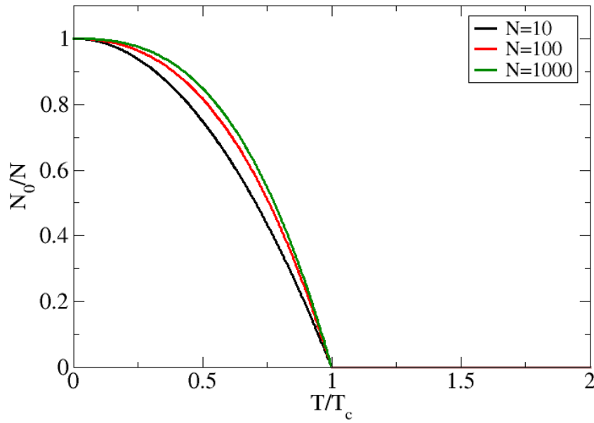
Figure 2.2: Condensate fraction for an isotropic three-dimensional harmonic trap in the semiclassical approximation calculated by Eq. (2.76) as a function of reduced temperature T/T_c^{(0)} with T_c^{(0)} given by Eq. (2.62) for a different number of particles N . The brown line in zero corresponds to all plots after the critical point due to, independently of N , the condensate fraction being zero for high temperatures in the grand canonical ensemble.
