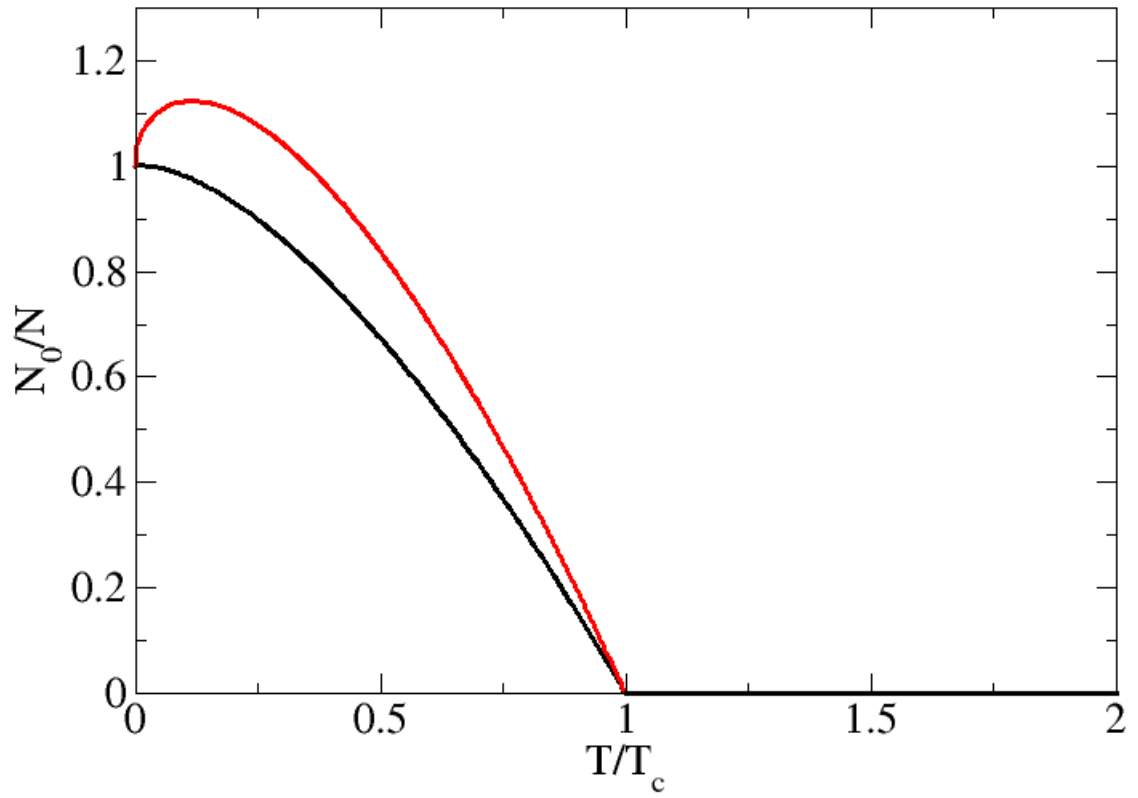
Figure 2.4: The comparison of the condensate fraction for 10 particles as a function of reduced temperature T/T_c^{(0)} with T_c^{(0)} given by Eq. (2.52) calculated by two formulas: the red line with Eq. (2.76) and the black line with Eq. (2.147). Is quite clear that this last formula corresponds to the correct formulation of our primary semi-classical approximation.
