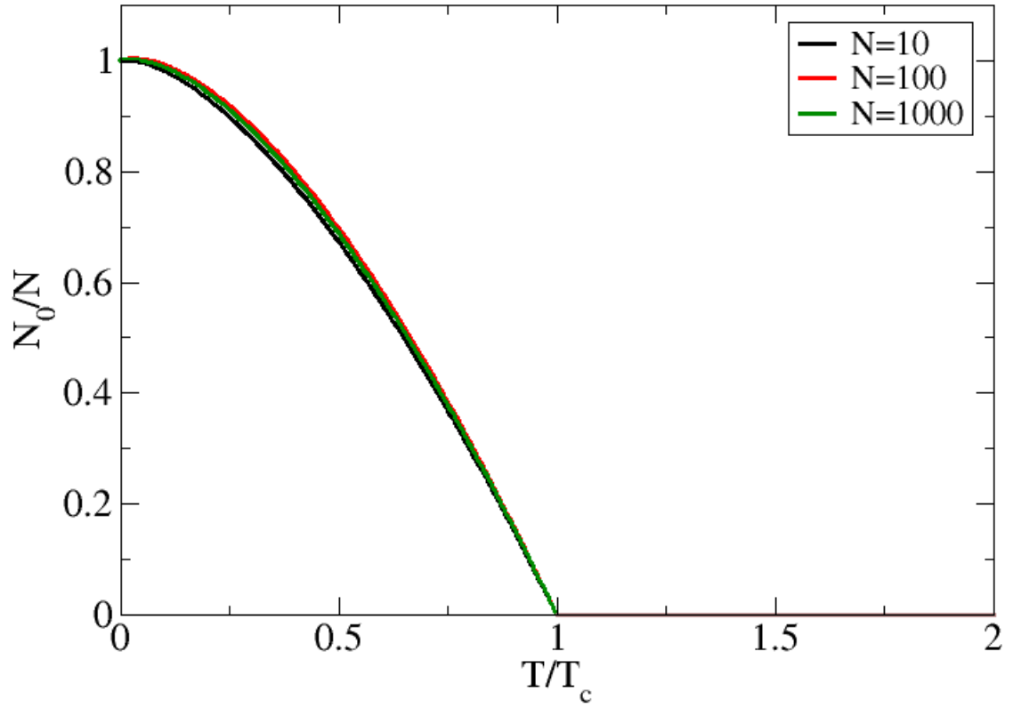
Figure 2.5: The condensate fraction of the three-dimensional finite box for 10, 100 and 1000 particles calculated by Eq. (2.147) as a function of reduced temperature T/T_c^{(0)} with T_c^{(0)} given by Eq. (2.52). The behavior is similar as seen in Fig. 2.3 but now the problem for a few particles in low temperatures was solved, therefore, we have the correct semi-classical approximation for the box trap.
