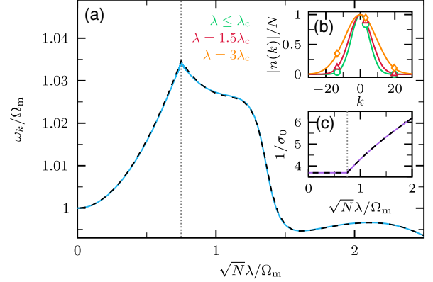
FIG. 4. (a) Membrane excitation frequency and (b) momentum distribution |n(k)| of the atoms in a single well. (c) Width of |n(k)| in dependence of \lambda . The dotted vertical line indicates \lambda_c . The parameters are V = 200\omega_R , \Omega_m = 100\omega_R , \gamma = 20\omega_R , and g = 0 .
