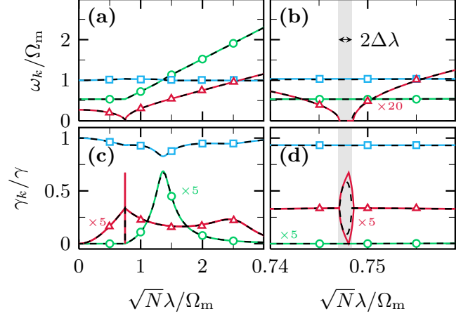
FIG. S2. (a), (b) Frequencies of collective excitations, and (c), (d) decay rates of the collective eigenmodes (some curves are scaled by the factors indicated). Panels (b) and (d) show a zoom around \lambda_c with width \Delta\lambda \simeq 0.1\omega_R . Different colors correspond to different eigenmodes. Curves in blue, green, and red correspond to the membrane mode, the condensate width mode, the atomic displacement excitation, correspondingly. The dashed curves show the GPE results. The parameters are V = 200\omega_R , \Omega_m = 100\omega_R , \gamma = 20\omega_R and g = 0 .
