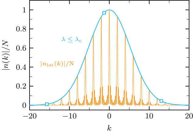
FIG. S3. Momentum distributions of atoms in a single lattice site |n(k)| , and of the full lattice n_{\text{lat}}(k) for M = 10 sites below the critical coupling \lambda_c . The parameters are V = 200\omega_R , \Omega_m = 100\omega_R , \gamma = 20\omega_R and g = 0 .
