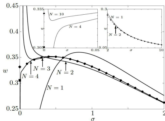
Figure 5. Regimes of synchronized and desynchronized dynamics. The phase boundary between the synchronized and desynchronized regimes is shown as a function of the noise strength \sigma . Areas below the curves correspond to the synchronized, areas above the curve to the desynchronized regime. The solid lines show the results of the first four Fourier orders, the dots represent numerical results. The diamond represents the coupling strengths for which the fixed point (\Phi_0, 0) of the deterministic system becomes unstable; the square indicates the value of w at which the stable limit cycle is first observed. The insets show results for small and for large noise. In the first inset (small noise) the results from the fourth and tenth Fourier orders are shown. The second inset (large noise) shows the results from the first (solid line) and second (dashed line) Fourier orders. Parameters are \omega = 1 , a = 1.2 .
