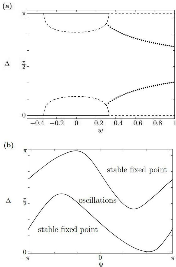
Figure 2. Stable and unstable fixed points and oscillations in the deterministic two-rotator system. (a) shows the bifurcation diagram with stable (solid lines) and unstable (dashed lines) fixed points of the system (27) for the choice of parameters \omega = 1 , a = 1.2 , w_{12} = w_{21} = w . Dots indicate the minimum and maximum values of oscillations in the value of \Delta that result for the initial conditions \Phi = 0 , \Delta = \pi/2 . (b) depicts for w = 0.308 the boundaries between the regions in the space of initial conditions for which the system converges to the limit cycle or the stable fixed point.
