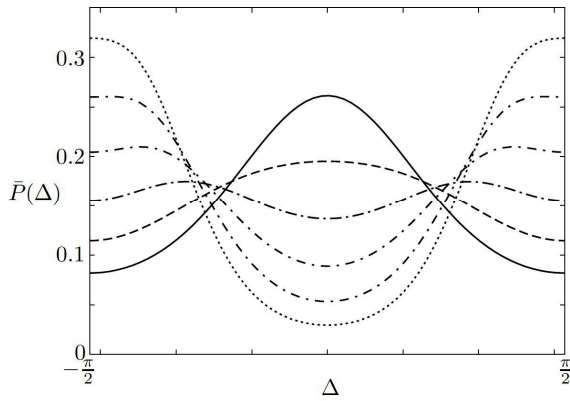
Figure 4. Marginal probability density for different values of the coupling strength w = w_{12} = w_{21} . The coupling strength for the curve with the highest value at \Delta = 0 (solid line) is w = 0.1 and increases from curve to curve in increments of \delta w = 0.2 to the maximum value w = 1.1 (dotted line). Other parameters are: \omega = 1 , \sigma = 0.4 , a = 1.2 .
