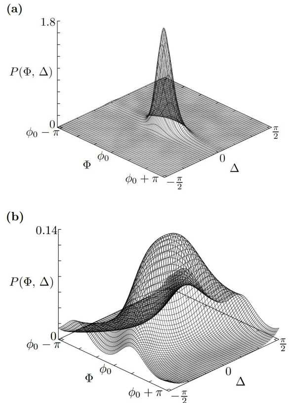
Figure 3. Synchronized and desynchronized modes in the stochastic two-rotator system. The stationary solution to the Fokker-Planck Equation (3) is shown for different values of the coupling strength. In both (a) and (b), we have w_{12} = w_{21} = w and \omega = 1 , a = 1.2 , \sigma = 0.4 . In (a) the coupling strength is w = 0.3 and the rotators are in a synchronized state; in (b) the coupling is increased to w = 0.4 and the two rotators desynchronize.
