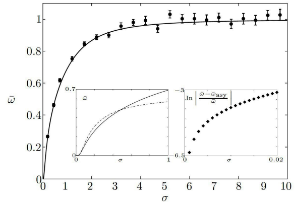
Figure 1. Average angular frequency of the single-rotator as a function of the noise intensity. The solid line shows the result (18). The dots represent results from Monte-Carlo simulations (mean \pm standard error of the mean) of the Langevin Equation (2). For each value of the noise intensity, forty runs were simulated up to T = 400 . The first inset shows a comparison between the asymptotic expansion (26, dashed line) and numerical evaluations of the expression (18, solid lines) for small noise. The diamonds in the second inset show the logarithm of the relative deviation between the result (18) and its asymptotic approximation (26). Parameters are: \omega = 1 , a = 1.2 .
