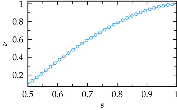
FIGURE 4.5: The critical exponent \nu is estimated as a function of the sub-Ohmic bath exponent s . The parameter were chosen as \omega_b = 0.5 \omega_a , \kappa = \omega_a , and \gamma = 0.25 \omega_a . The data points are taken from reference [199].
