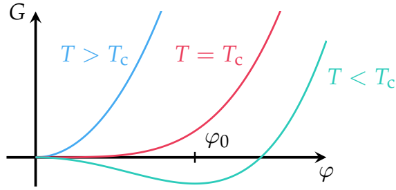
FIGURE 4.1: The schematic behavior of the free enthalpy G is shown as a function of the order parameter for three different temperatures.
