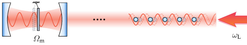
FIGURE 5.1: A nanomechanical membrane inside an optical cavity is coupled to the vibrational motion of a distant atomic ensemble.
