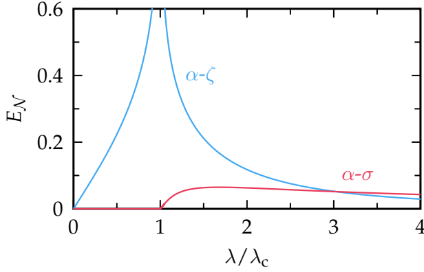
FIGURE 6.8: The logarithmic negativity E_N is shown as a function of the atom-membrane coupling \lambda . The blue (red) curve measures the entanglement between membrane displacement and condensate displacement (width) mode. The same parameters as in figure 6.6 have been used, but with \Gamma_m = 0 .
